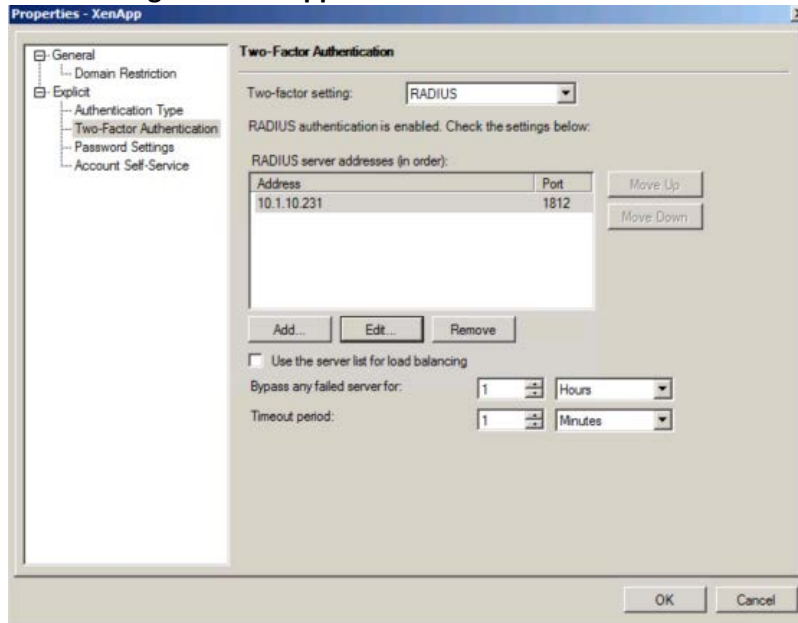
Figure 2. XenApp Two-Factor Authentication 43
