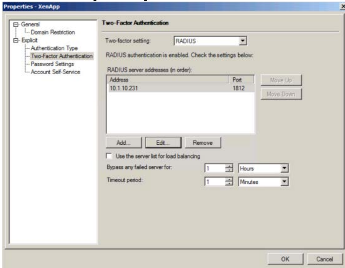
Figure 3. Adding the Radius Server IP Address 44
