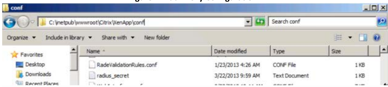
Figure 4. AuthProxy Configuration 45
